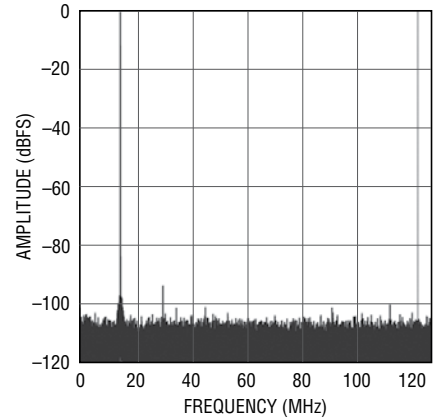
LTC2152-14: 32K Point FFT, f_{IN} = 15\text{MHz} , -1\text{dBFS} , 250\text{Mps}
