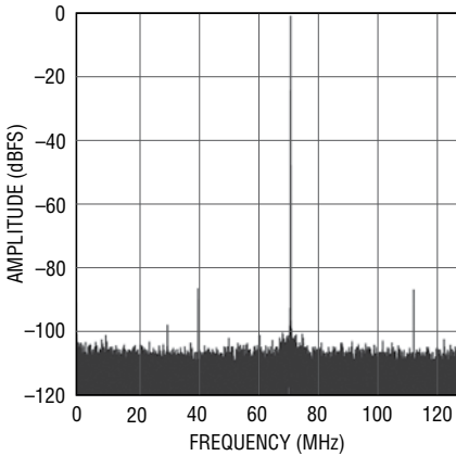
LTC2152-14: 32K Point FFT, f_{IN} = 70\text{MHz} , -1\text{dBFS} , 250\text{Mps}
