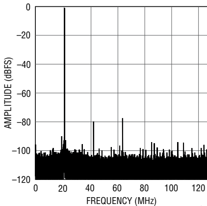
LTC2152-14: 32K Point FFT, f_{IN} = 229\text{MHz} , -1\text{dBFS} , 250\text{Mps}
