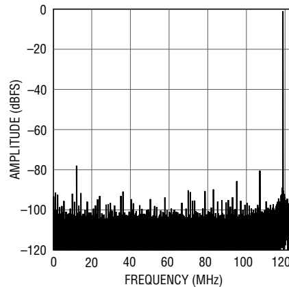
LTC2152-14: 32K Point FFT, f_{IN} = 381\text{MHz} , -1\text{dBFS} , 250\text{Mps}
