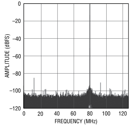
LTC2152-14: 32K Point FFT, f_{IN} = 171\text{MHz} , -1\text{dBFS} , 250\text{Mps}
