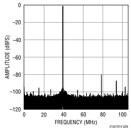
LTC2151-14: 32K Point FFT, f_{IN} = 171\text{MHz} , -1\text{dBFS} , 210MSPs
