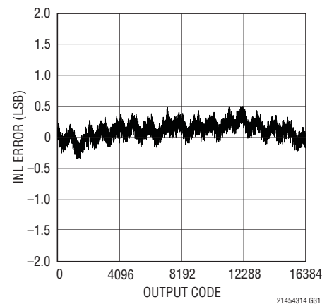
LTC2143-14: Integral Nonlinearity (INL)
