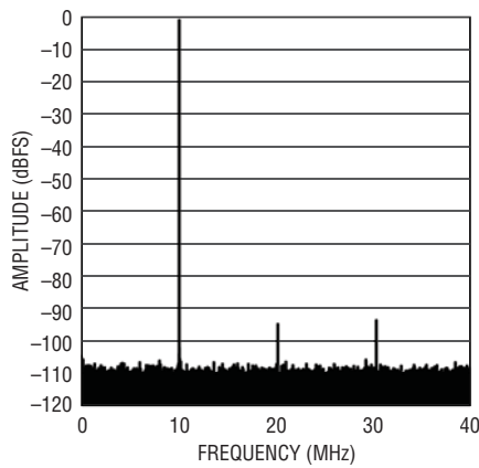
LTC2143-12: 64k Point FFT, f_{IN} = 70\text{MHz} , -1dBFS, 80Msps
