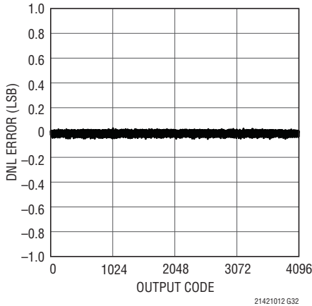
LTC2140-12: Differential Non-Linearity (DNL)
