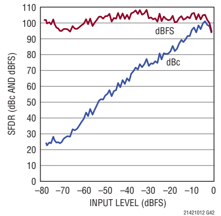
LTC2140-12: SFDR vs Input Level, f_{IN} = 70\text{MHz} , 25\text{Mpsps} , 2\text{V} Range
