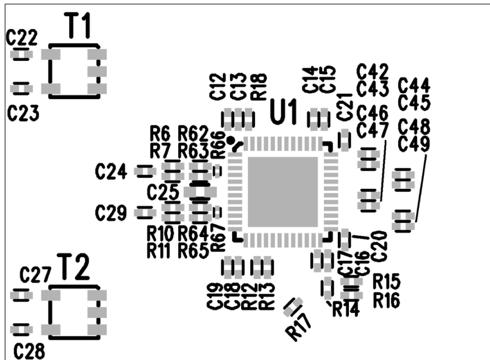
Silkscreen Top
