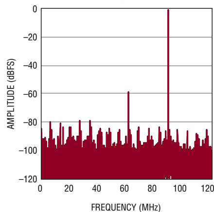
64k Point FFT, f_{IN} = 907.1\text{MHz} , -1dBFS, 250Mps
