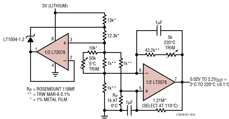
Platinum RTD Signal Conditioner with Curvature Correction
