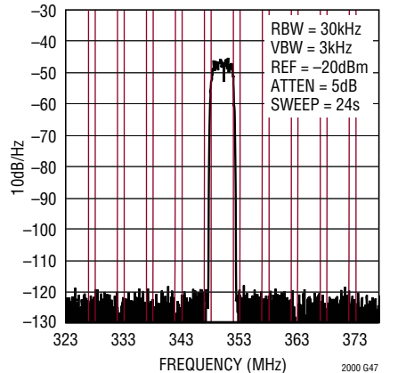
LTC2000-16 Single Carrier WCDMA ACLR at 350MHz, f_{DAC} = 2.5Gps
