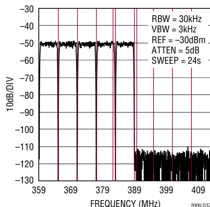
32-Carrier DOCSIS Low Band Narrowband ACLR, f_{DAC} = 2.5Gsp
