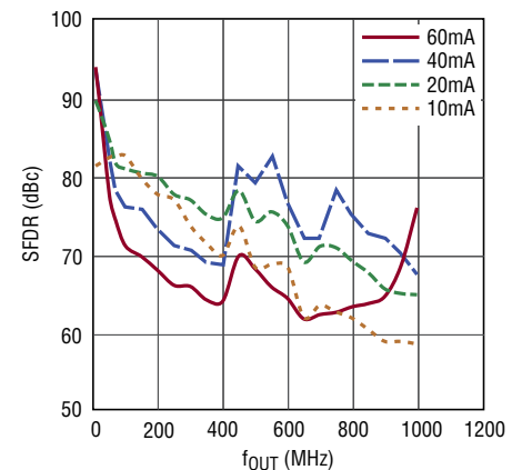
SFDR vs f_{OUT} and I_{OUTFS} , f_{DAC} = 2.5\text{Gsp/s}
