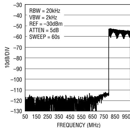
32 Carrier DOCSIS High Band Wideband ACLR, f_{DAC} = 2.5Gsp
