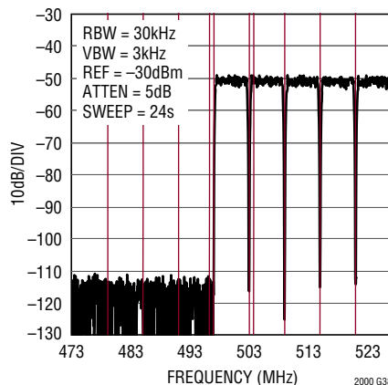
32 Carrier DOCSIS Mid Band Narrowband ACLR, f_{DAC} = 2.5Gsp
