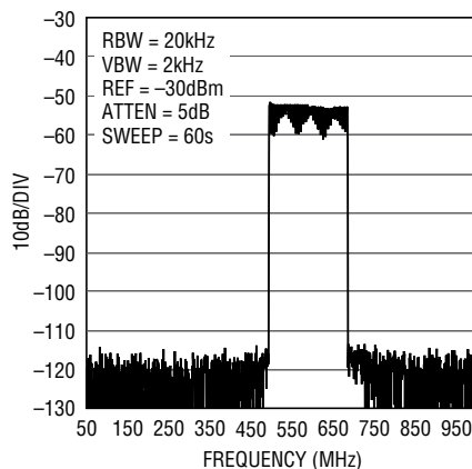
32-Carrier DOCSIS Mid Band Wideband ACLR, f_{DAC} = 2.5Gsp
