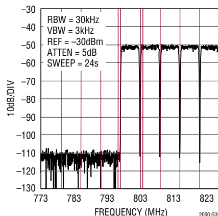
32 Carrier DOCSIS High Band Narrowband ACLR, f_{DAC} = 2.5Gsp
