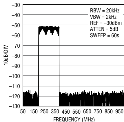
32-Carrier DOCSIS Low Band Wideband ACLR, f_{DAC} = 2.5Gsp
