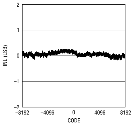
LTC2000-14 Integral Nonlinearity (INL)
