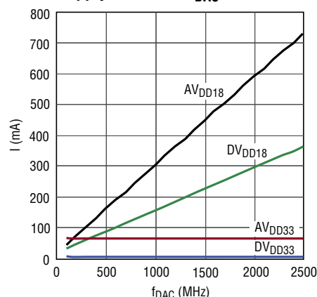
Supply Current vs f_{DAC}
