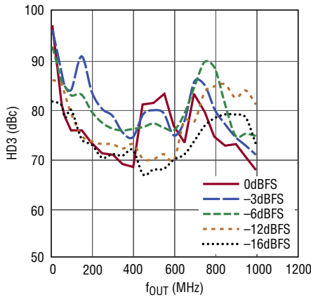
HD3 vs f_{OUT} and Digital Amplitude (dBFS), f_{DAC} = 2.5\text{Gpsps}
