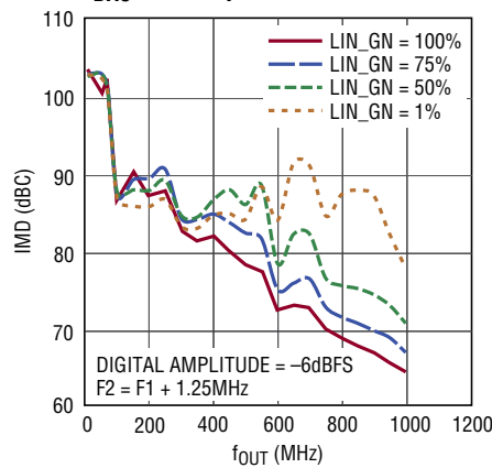
2-Tone IMD vs f_{OUT} and Linearization Setting, f_{DAC} = 2.5\text{Gpsps}
