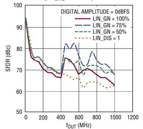
SFDR vs f_{OUT} and Linearization Setting, f_{DAC} = 2.5\text{Gpsps}
