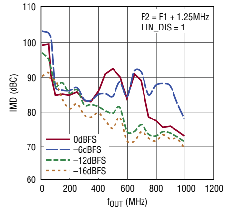
2-Tone IMD vs f_{OUT} and Digital Amplitude, f_{DAC} = 2.5\text{Gpsps}
