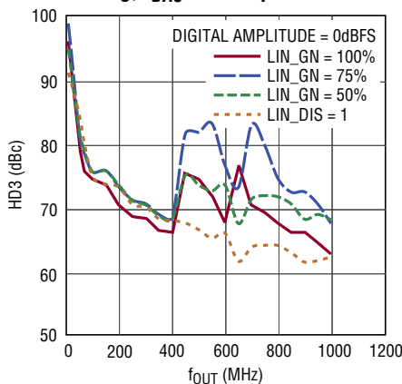
HD3 vs f_{OUT} and Linearization Setting, f_{DAC} = 2.5\text{Gpsps}
