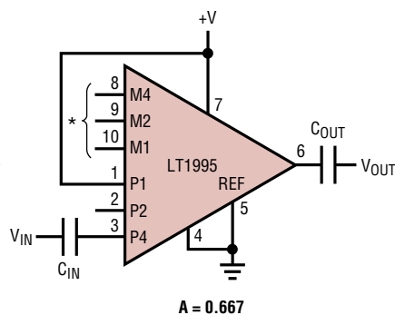
Figure 7. AC-Coupled Noninverting Amplifier Input Attenuation Configurations (Supply Splitting)
