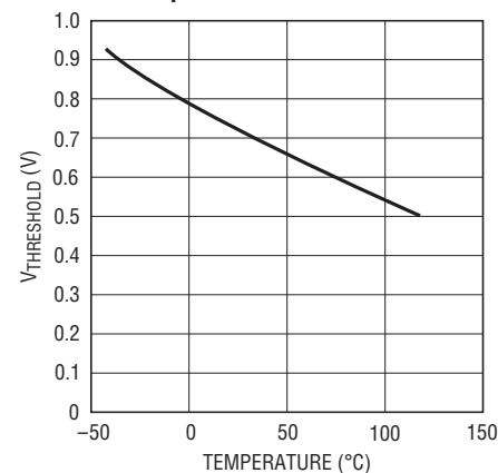
\overline{SHDN} Pin Threshold Voltage vs Temperature
