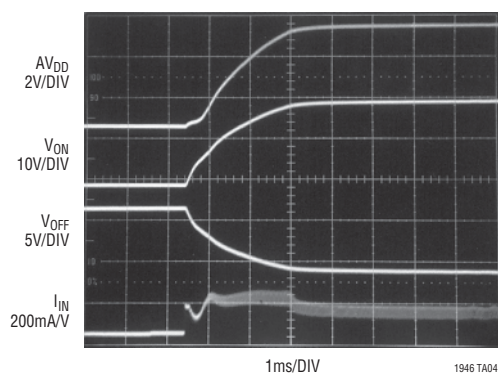
Start-Up Waveforms
