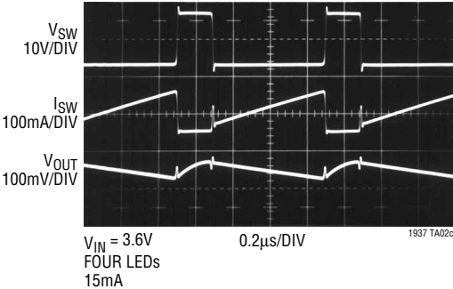
Switching Waveforms
