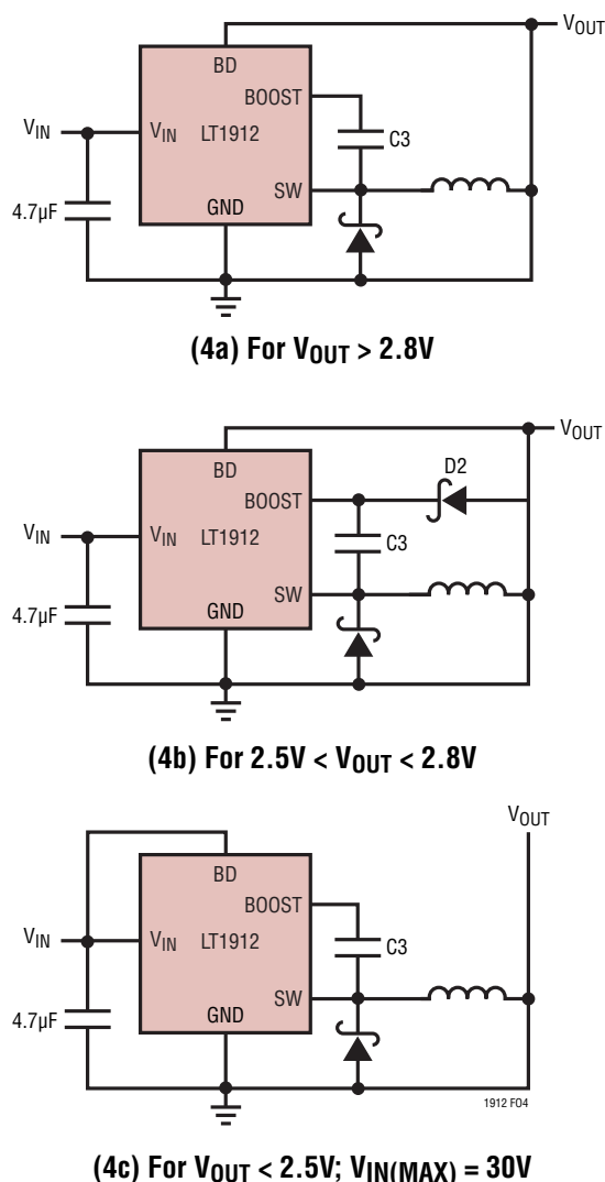
Figure 4. Three Circuits For Generating The Boost Voltage
