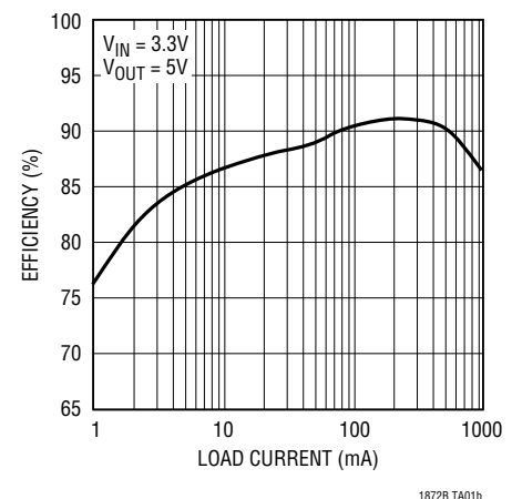
Typical Efficiency vs Load Current*
