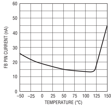
FB Pin Current vs Temperature
