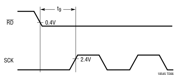
t_9 ( \overline{RD} \downarrow to SCK Setup Time)
