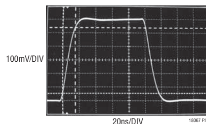
Figure 11. Step Response with R_F = 499\text{k}
