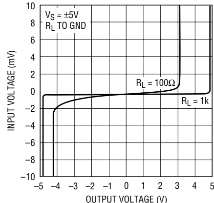
Open-Loop Gain
