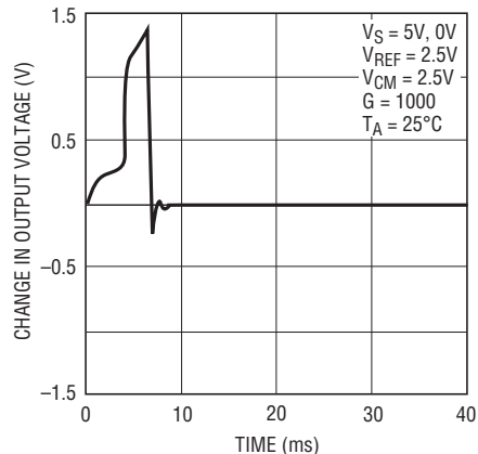
Turn-On Characteristics
