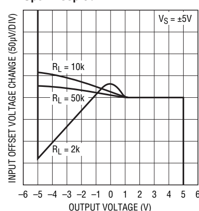
Open-Loop Gain
