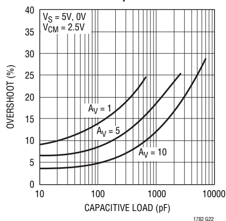
Capacitive Load Handling Overshoot vs Capacitive Load
