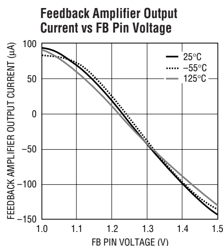
LT1776 G11
