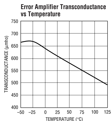
LT1776 G12
