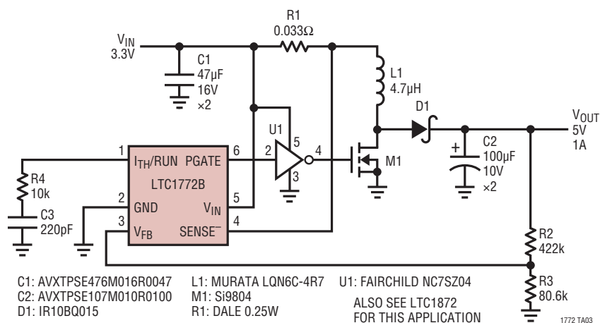
LTC1772B 3.3V to 5V/1A Boost Regulator
