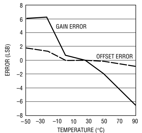
Offset and Gain Error vs Temperature
