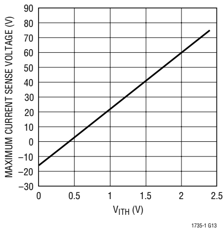
Maximum Current Sense Voltage vs I_{\text{TH}} Voltage
