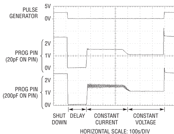
Figure 5. Stability Waveforms
