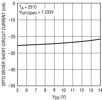
Opto Driver Short-Circuit Current vs V_{DD}
