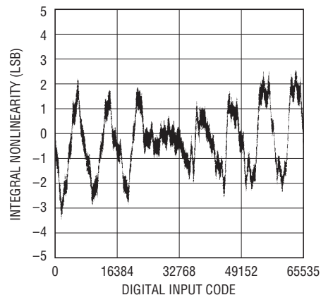
LTC1657 Integral Nonlinearity
