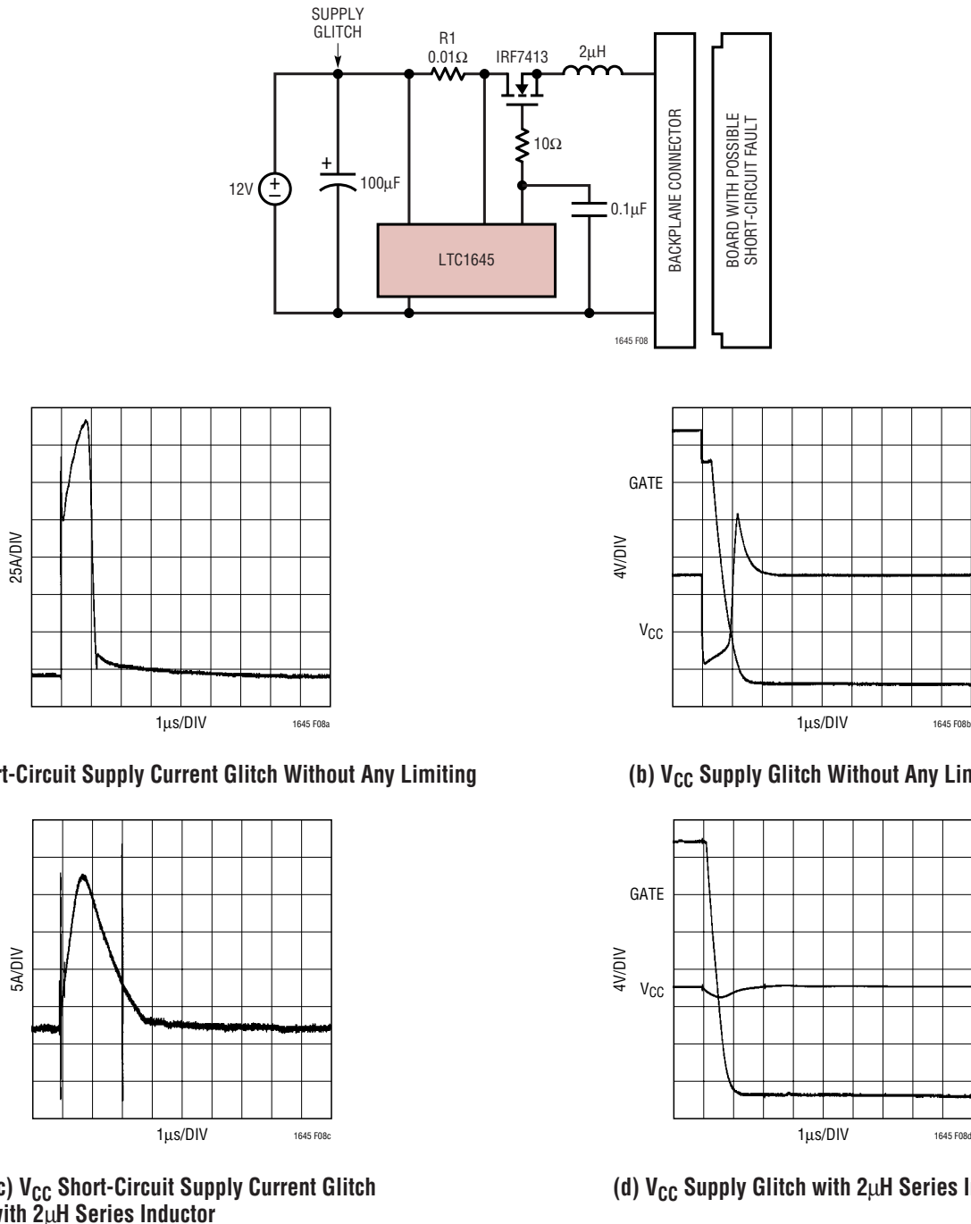
Figure 8. Supply Glitch
