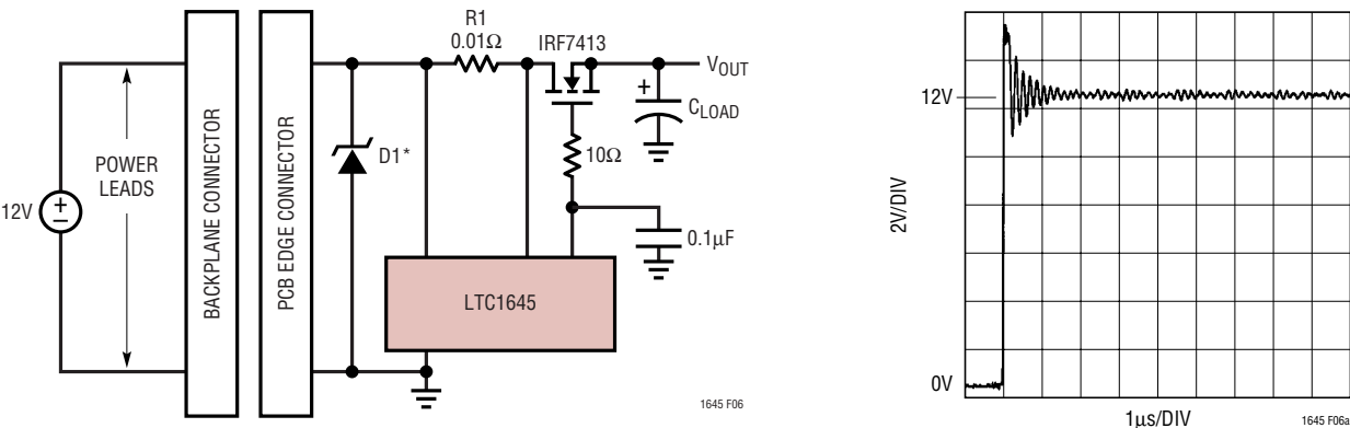
V CC Waveform Clamped by a Transient Suppressor
