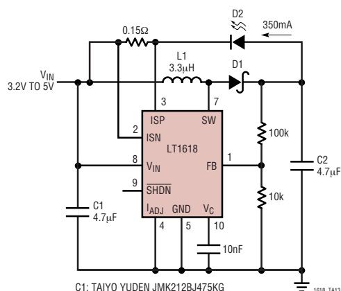
Li-Ion Buck-Boost Mode Luxeon LED Driver
