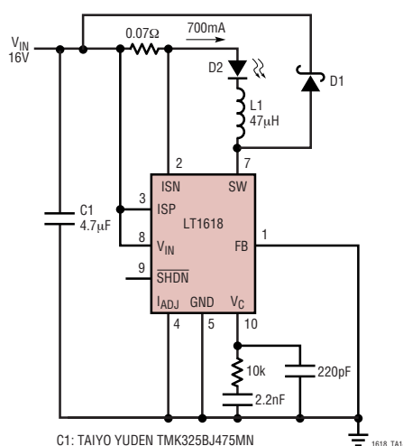
Buck Mode Luxeon LED Driver
