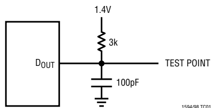
Load Circuit for t_{dPO} , t_r and t_f
