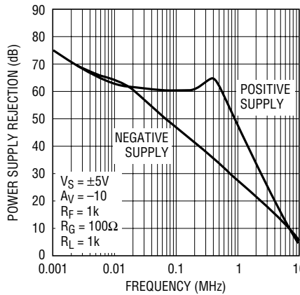
PSRR of OA vs Frequency
