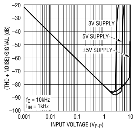
THD + Noise vs Input Voltage ( f_C = 10\text{kHz} )
