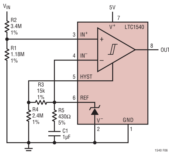
Figure 6. Glitch-Free Level Detector with Hysteresis
