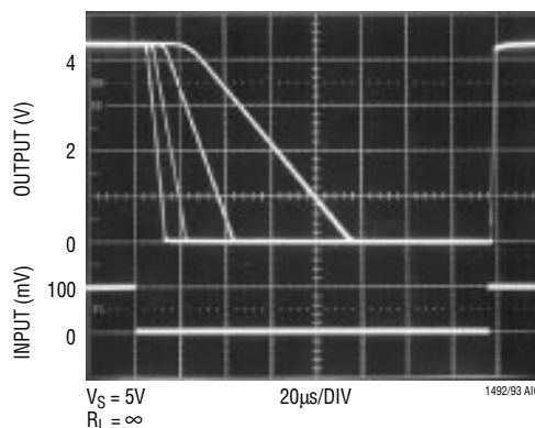
Comparator Response (-) 20mV, 10mV, 5mV, 2mV Overdrives
