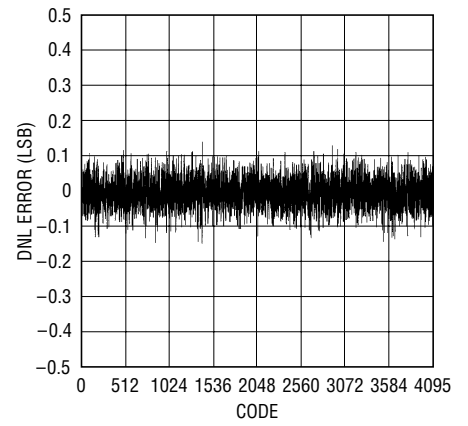
LTC1446L Differential Nonlinearity
