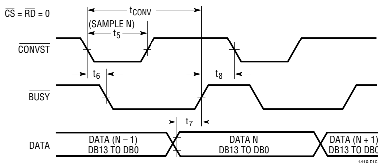
Figure 16. Mode 1a. \overline{\text{CONVST}} Starts a Conversion. Data Outputs Always Enabled ( \overline{\text{CONVST}} = narrow pulse)
