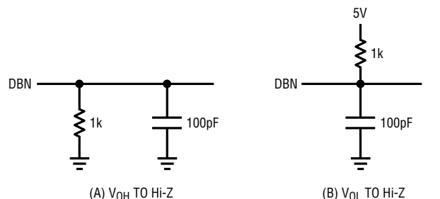
Load Circuits for Output Float Delay
