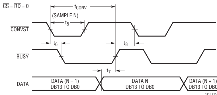
Figure 15. Mode 1a. \overline{CONVST} Starts a Conversion. Data Outputs Always Enabled ( \overline{CONVST} = \text{low} )
