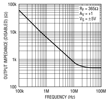
Output Impedance (Disabled) vs Frequency
