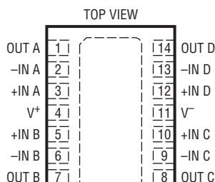
DE14 PACKAGE 14-LEAD (4mm x 3mm) PLASTIC DFN T_{JMAX} = 150^\circ\text{C} , \theta_{JA} = 43^\circ\text{C/W} , \theta_{JC} = 4.3^\circ\text{C/W} EXPOSED PAD (PIN 15) IS V^- MUST BE SOLDERED TO PCB
