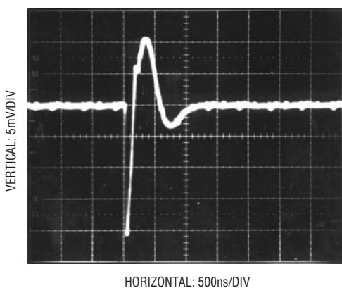
Figure 10. Adequate Settling of Op Amp Driving Analog Input
