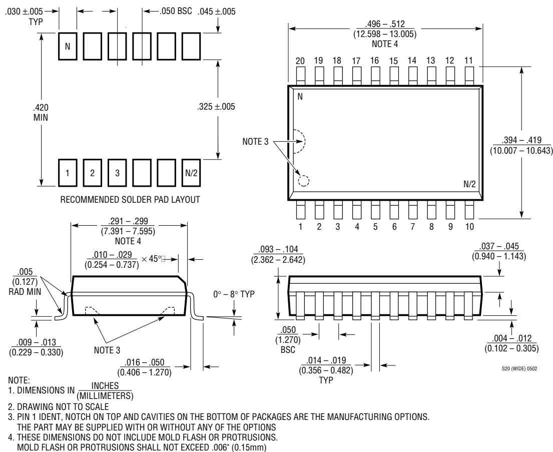
SW Package 20-Lead Plastic Small Outline (Wide .300 Inch) (Reference LTC DWG # 05-08-1620)
