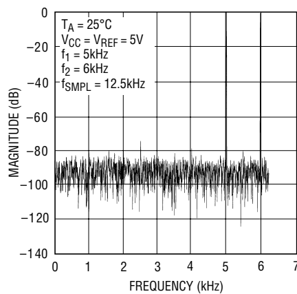
Intermodulation Distortion
