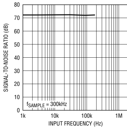
Signal-to-Noise Ratio (Without Harmonics) vs Input Frequency
