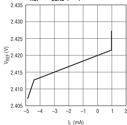
V REF vs I LOAD (mA)
