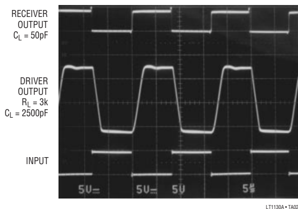
Output Waveforms
