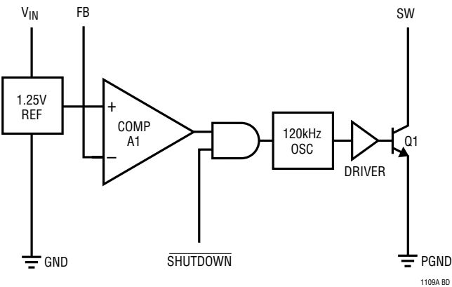
LT1109A (Adjustable)
