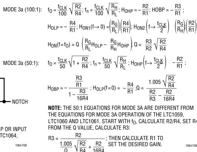
Figure 9. Mode 3a: 2nd Order Filter Providing Highpass, Bandpass, Lowpass and Notch
